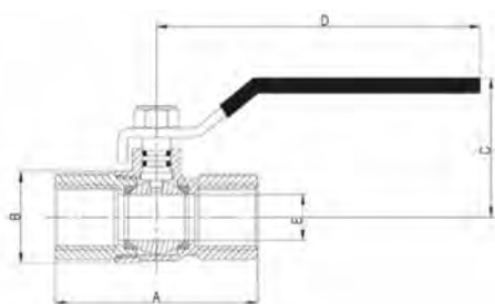
Brass Ball Valve - FI x FI
