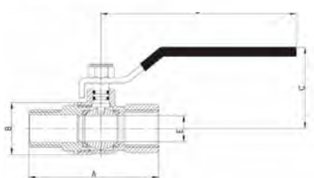
Brass Ball Valve - MI x FI
