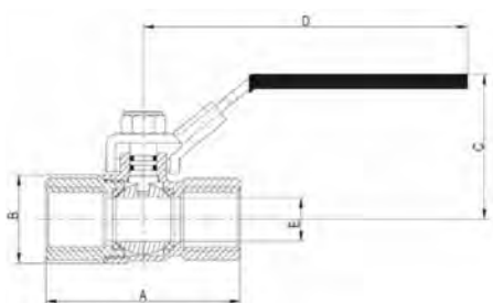
Brass Ball Valve - Lockable - FI x FI
