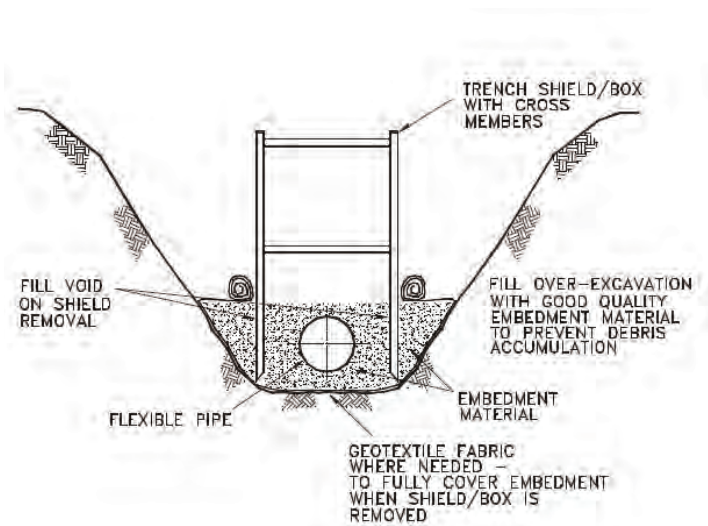
FIGURE 4.4 Shields in wide trench
