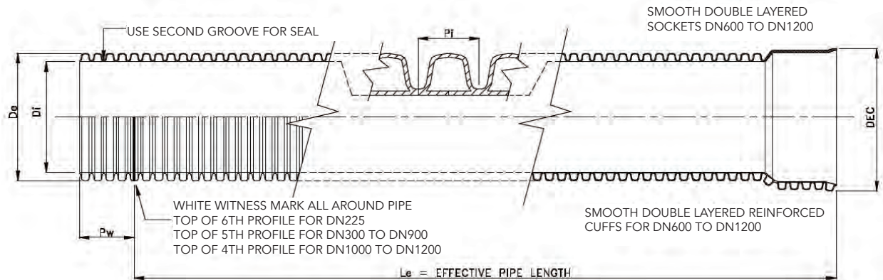
FIGURE 2.1 BlackMax Pipe – Longitudinal Cross-Section
