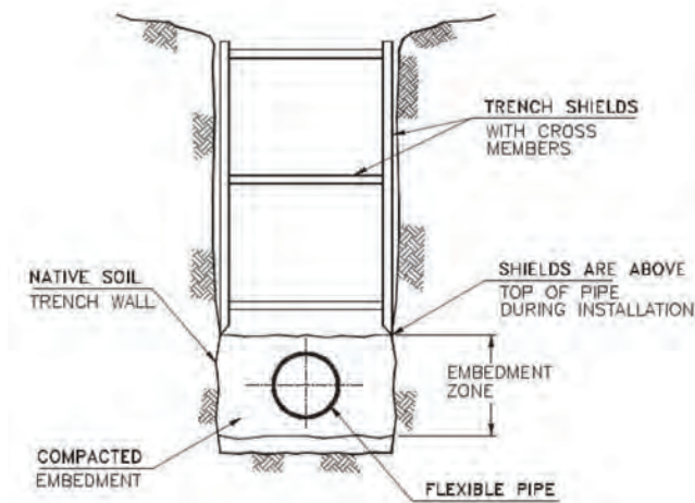
FIGURE 4.2 Shields kept above side support
