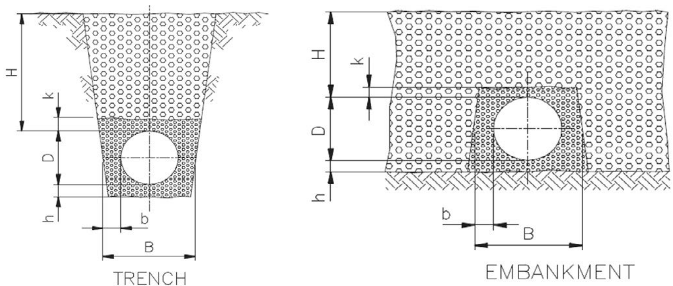
FIGURE 3.8 Critical dimensions for design and installation
