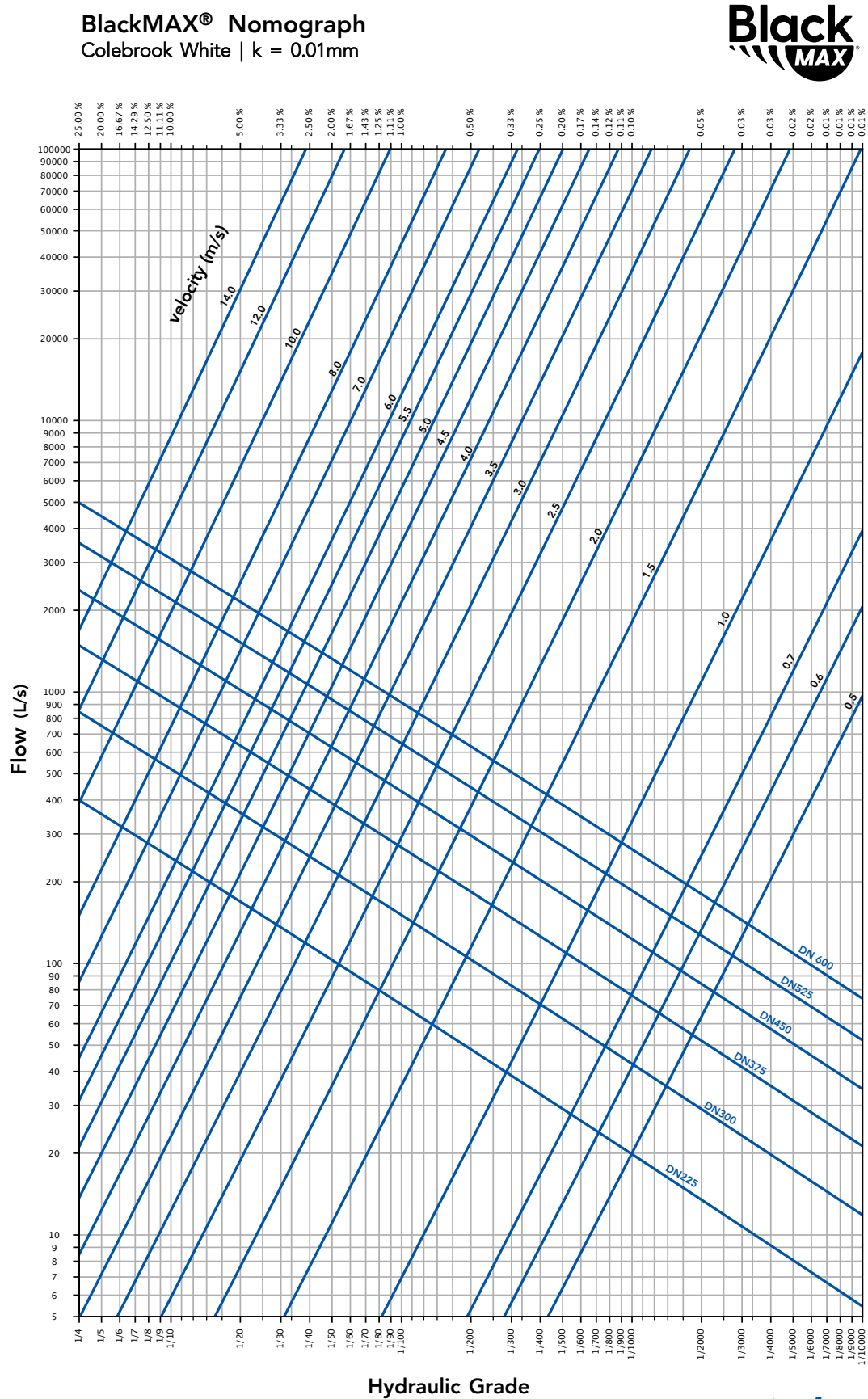
FIGURE 3.1 Colebrook White Flow chart used typically for Stormwater drainage applications k=0.01\text{mm}
