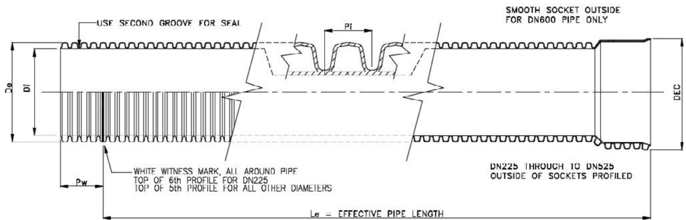
FIGURE 2.1 BlackMAX® Pipe – Longitudinal Cross-Section
