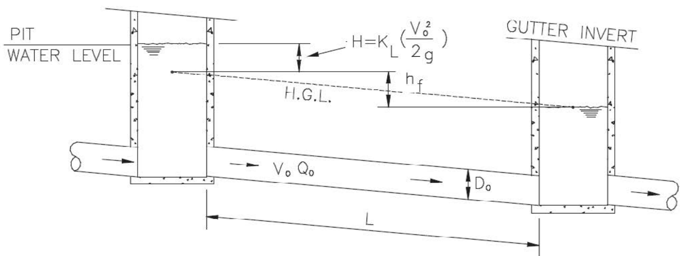
Figure 3.5 Head losses through Stormwater pits
