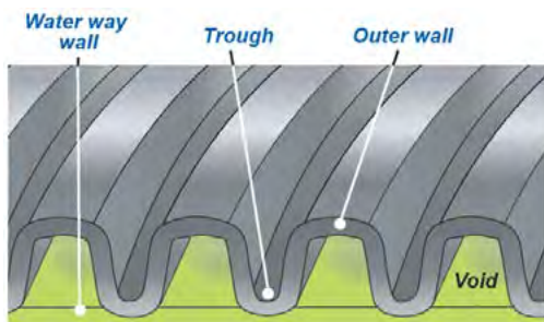
Figure 1.1 Cross sections of Iplex PP structured wall pipe systems
