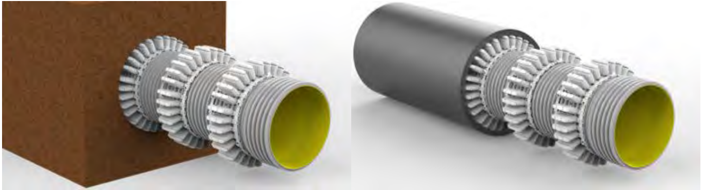
FIGURE 4.5 Approved Plastic Spacer Arrangement for SewerMAX® pipes
