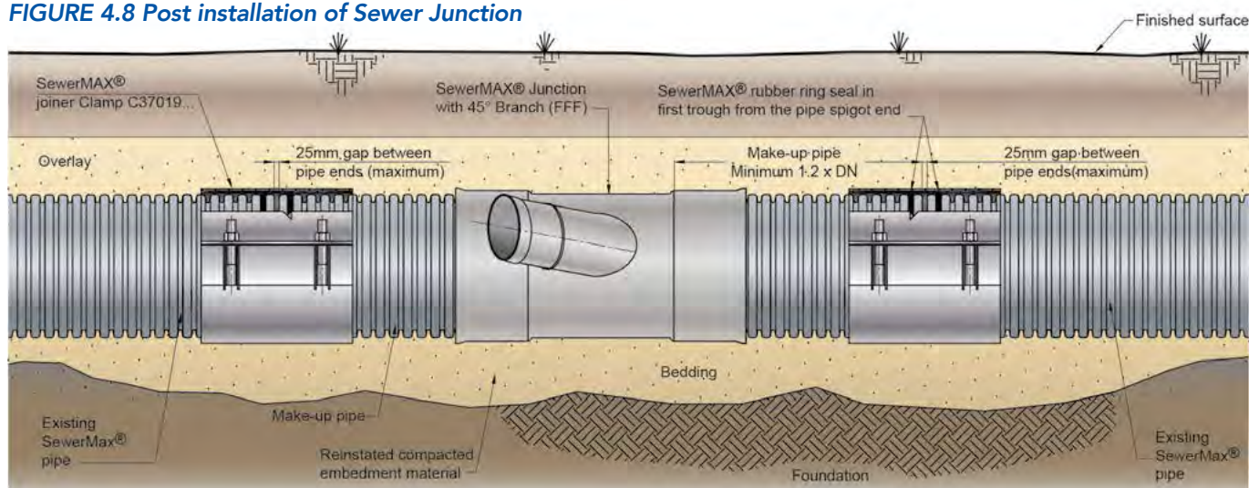
Post installation of SewerMAX® Junction (FFF) with SewerMAX® Joiner Clamps
