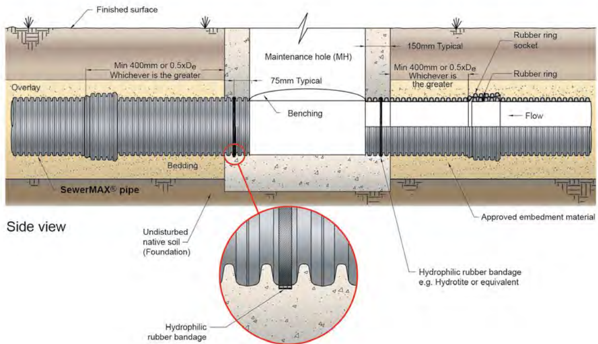
FIGURE 4.7 Typical connection to a concrete sewer maintenance hole MH with SewerMAX® pipe
