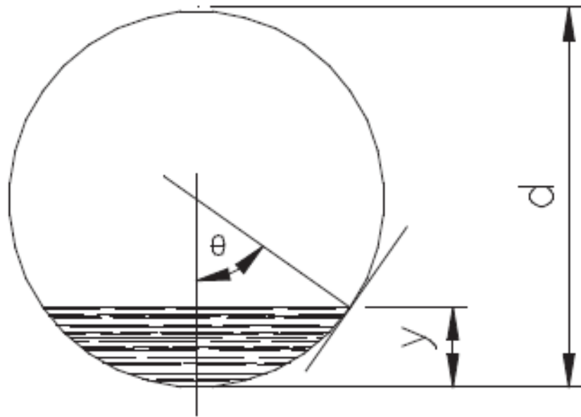
Figure 3.6 Angle of repose of sediment for a self-cleansing flow
