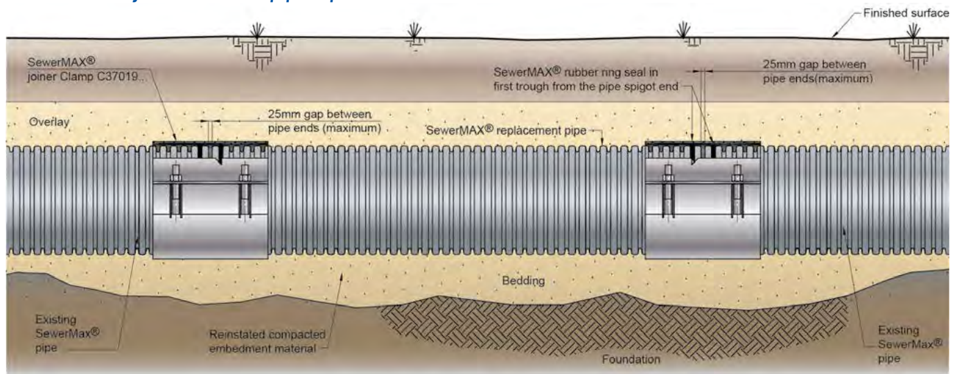
FIGURE 4.9 Major SewerMAX® pipe repair
