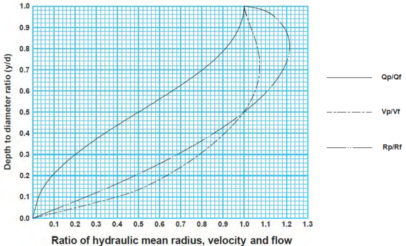
FIGURE 3.7 Proportional velocity and discharge in part-full pipes
