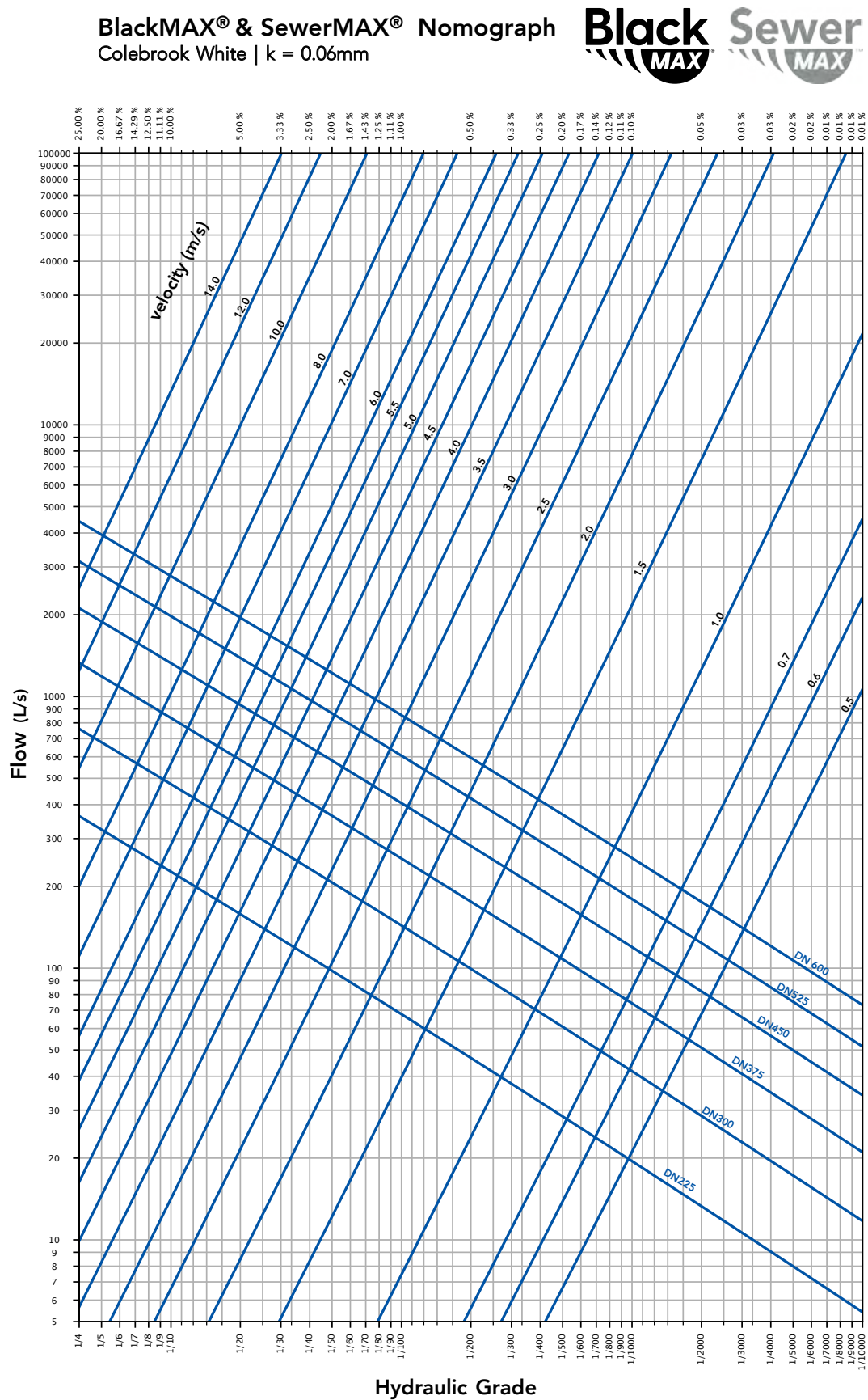
FIGURE 3.2 Colebrook White Flow chart used typically for Stormwater drainage and Sewer applications k=0.06\text{mm}
