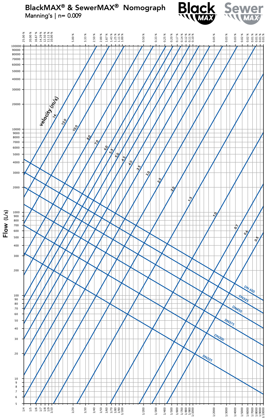
FIGURE 3.4 Manning's Flow chart used typically for Stormwater drainage and Sewer applications n=0.009
